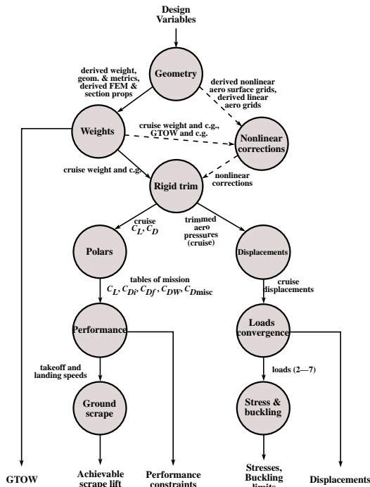
Fig. 7 Analysis process.
