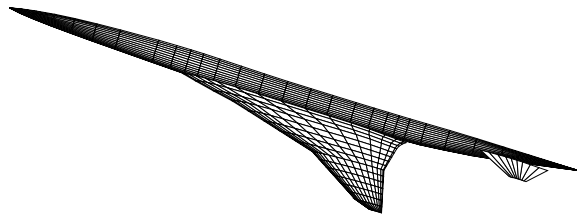
a) Linear aerodynamic grid
