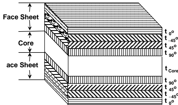
Fig. 4. Composite laminate stacking sequence.
