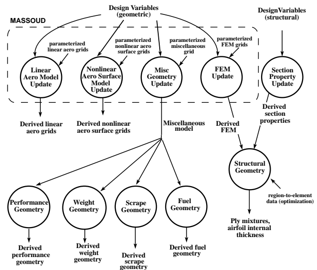
Fig. 8 Geometry Process.
